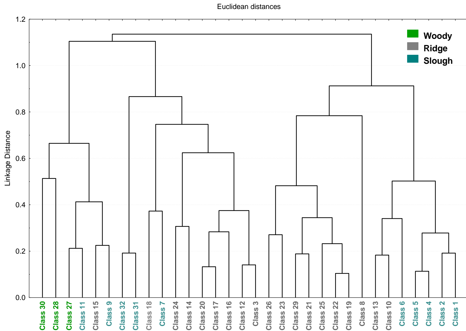
Figure 5: Dendrogram of ISODATA clustering algorithm for PSU 4 with a a posteriori classification.
